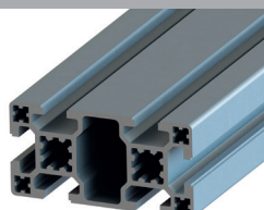
40x80 Slotpro 6 Slot Standard Profile
