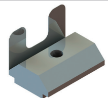
4 Series Roll in Slot Nut M4
