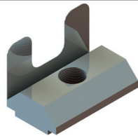
3 Series Roll in Slot Nut M6
